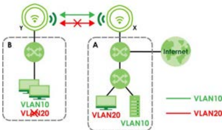
Figure 11 Wireless Bridge (with VLAN10)
