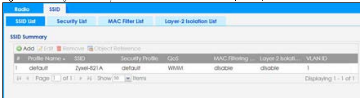
Figure 113 Configuration > Object > AP Profile > SSID > SSID List (After wizard setup)
