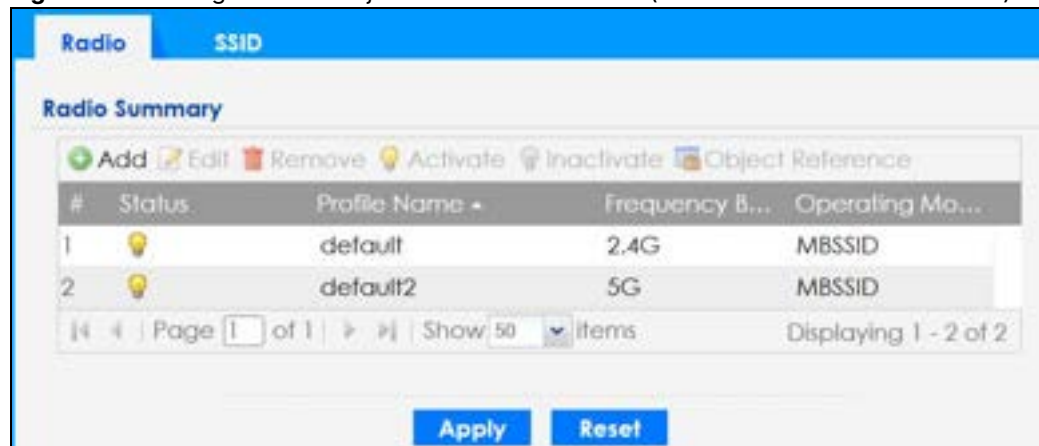
Figure 108 Configuration > Object > AP Profile > Radio (for 2.4 GHz and 5 GHz models)
