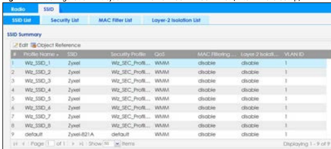
Figure 113 Configuration > Object > AP Profile > SSID > SSID List (After wizard setup)
