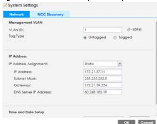
Figure 177 Dashboard > Edit (System Status) > Network
