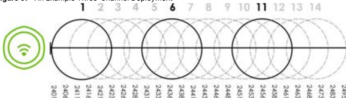
Figure 97 An Example Three-Channel Deployment
