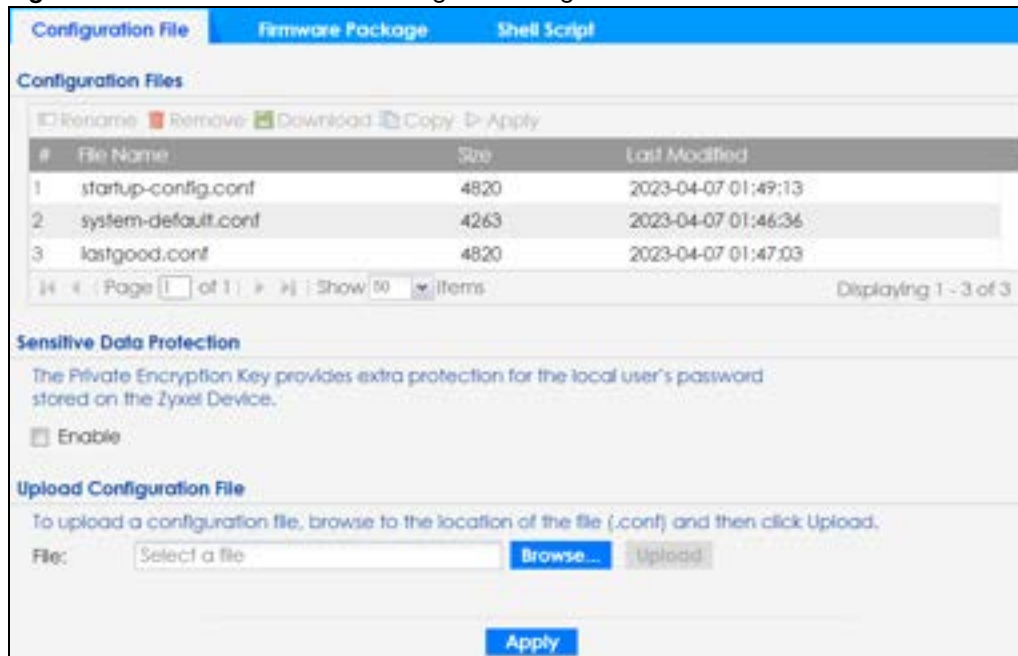
Figure 158 Maintenance > File Manager > Configuration File
