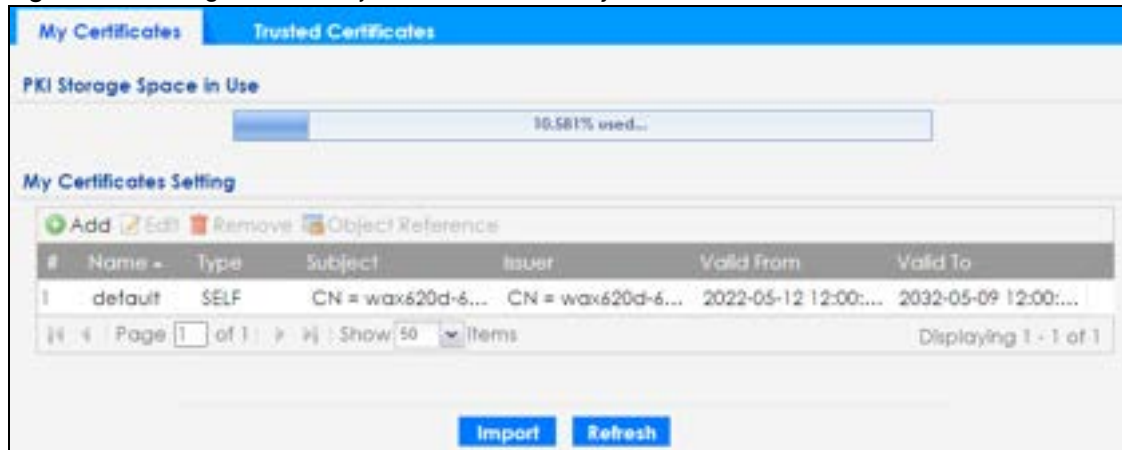
Figure 131 Configuration > Object > Certificate > My Certificates
