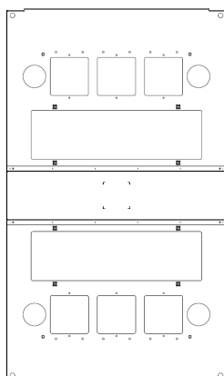
Top Panel 2off 130 x 448mm 6off 100 x 100mm 4off 60mm diameter
