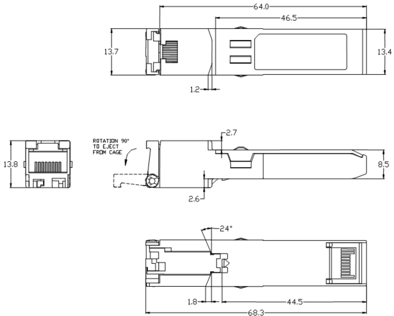
Figure 2. Mechanical Dimensions of Transceiver
