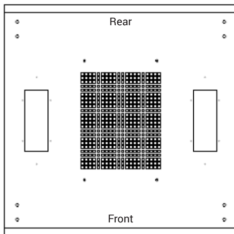
Top Panel 600W x 600D
