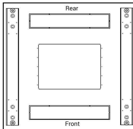
Bottom Panel 600W x 600D
