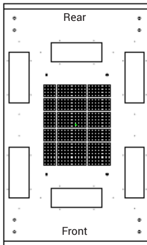
Top Panel 600W x 1200D
