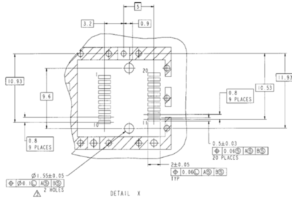
Figure 3. SFP Host Board Mechanical Layout
