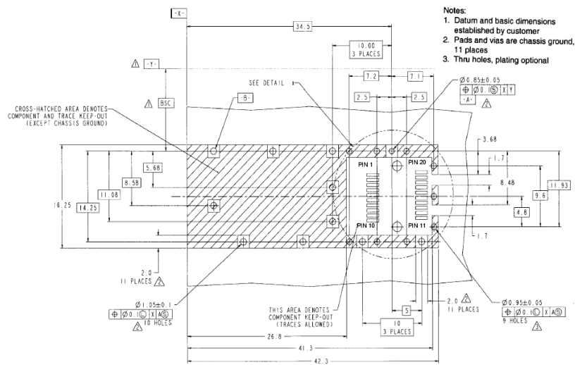
Figure 3. SFP Host Board Mechanical Layout
