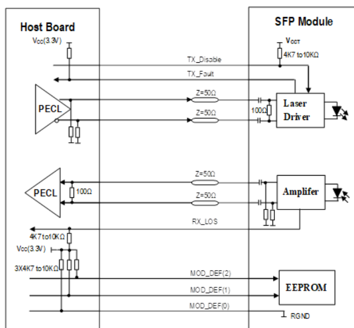
Figure 5. SFP Host Recommended Circuit
