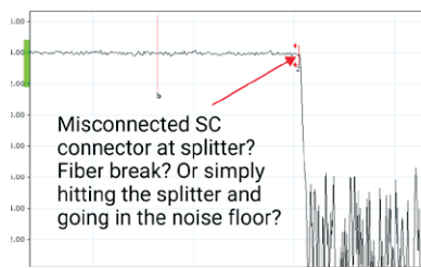
Figure 2. Last-Mile OTDR trace.
