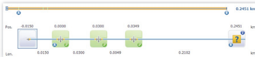
Figure 3. Test fail—Expected splitter not detected. Last mile looks OK but there is either a break or disconnection at splitter.
