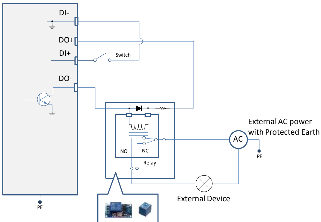
Dry contact and using camera's DO+ to supply a relay.
