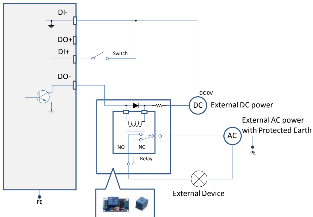
Wet contact with external DC power source to supply a relay.
